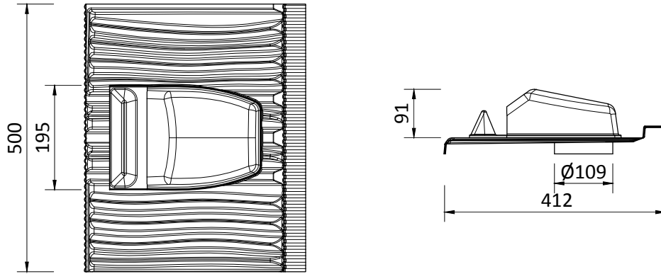
Figure 1.1 Vent Dimensions
