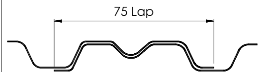
Figure 1.4 Lap Section
