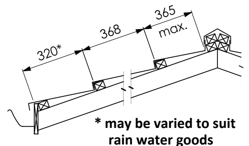
Figure 1.5 Batten Layout
